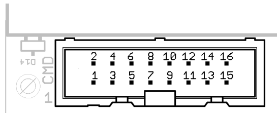
Figure 7: CMD connector (8x2 0.1" centers shrouded header)
