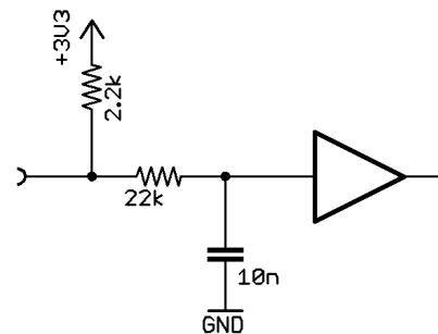
Figure 6: Equivalent circuit for Hall sensor inputs (pins 1-3)
