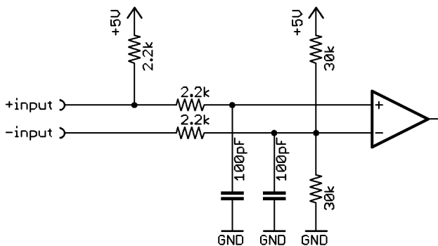
Figure 5: Equivalent circuit for differential inputs (pins 4-7 and 12-15)
