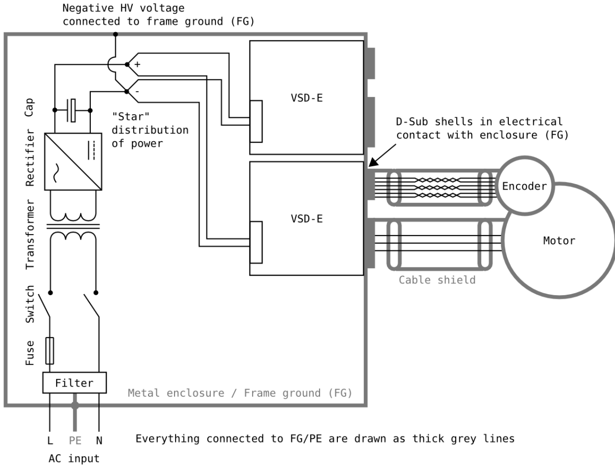
Figure 12: Suggested VSD-E installation scheme
