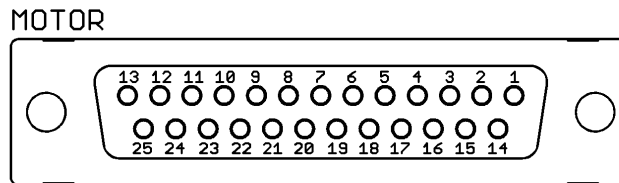
Figure 3: Motor connector pin out (25 pin female D-Sub)
