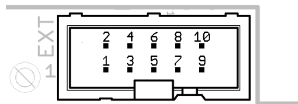
Figure 11: EXT connector (5x2 0.1" centers shrouded header)
