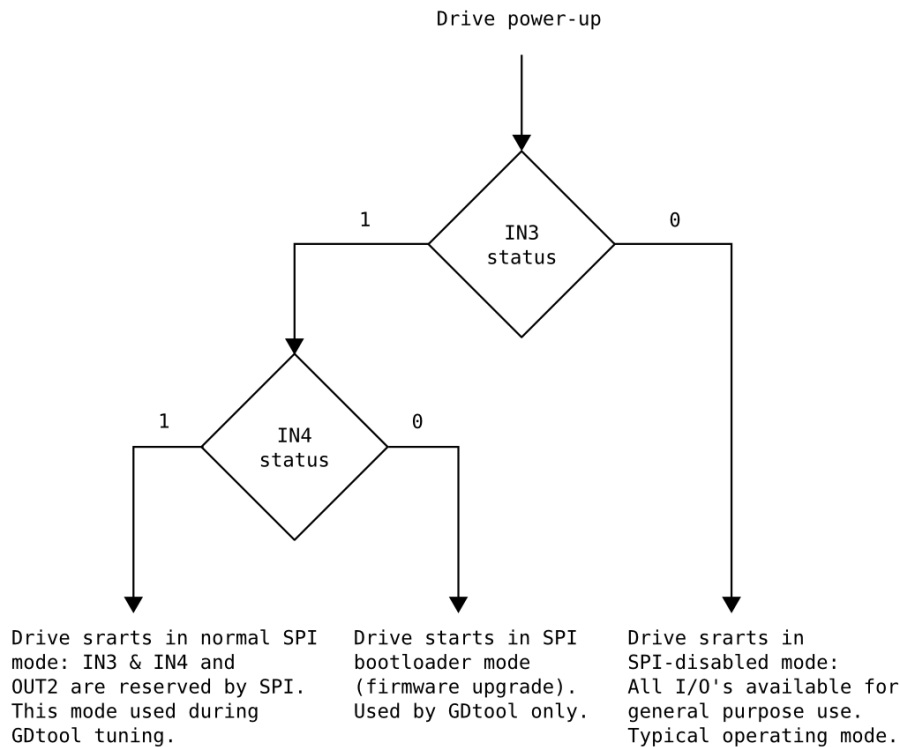
Figure 16: Operation mode selection during logic voltage rise versus CMD port IN3 & IN4 logic statuses
