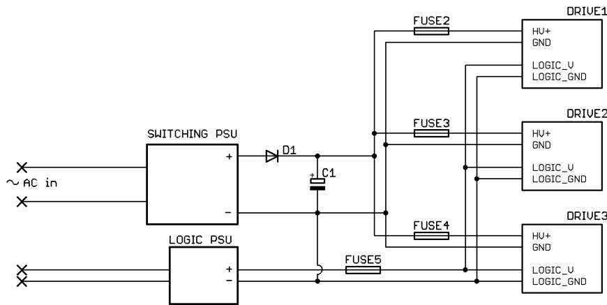
Figure 15: Switching mode power supply (SMPS) circuit
