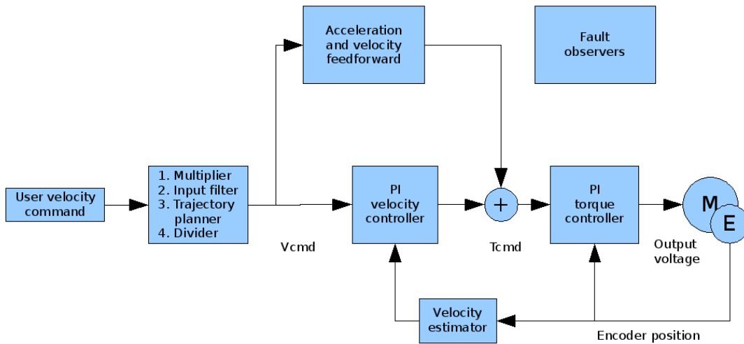
Figure 17: Overview block diagram of PI type velocity controller.
