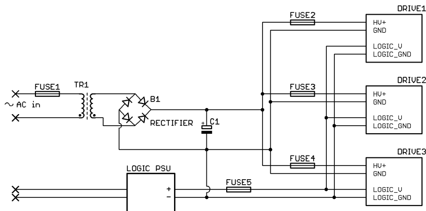
Figure 14: Simple transformer based linear PSU up to about 500 Watts
