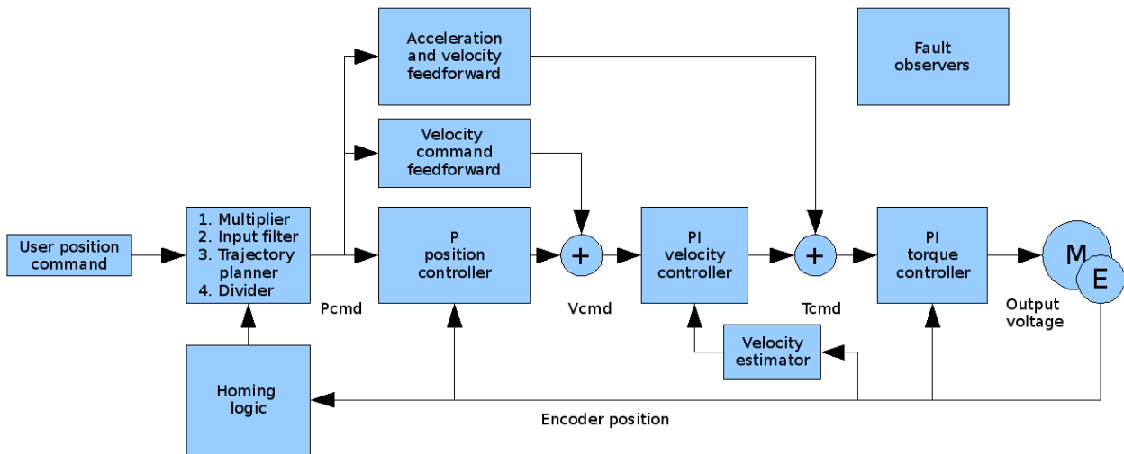
Figure 18: Overview block diagram of PIV type position controller.
