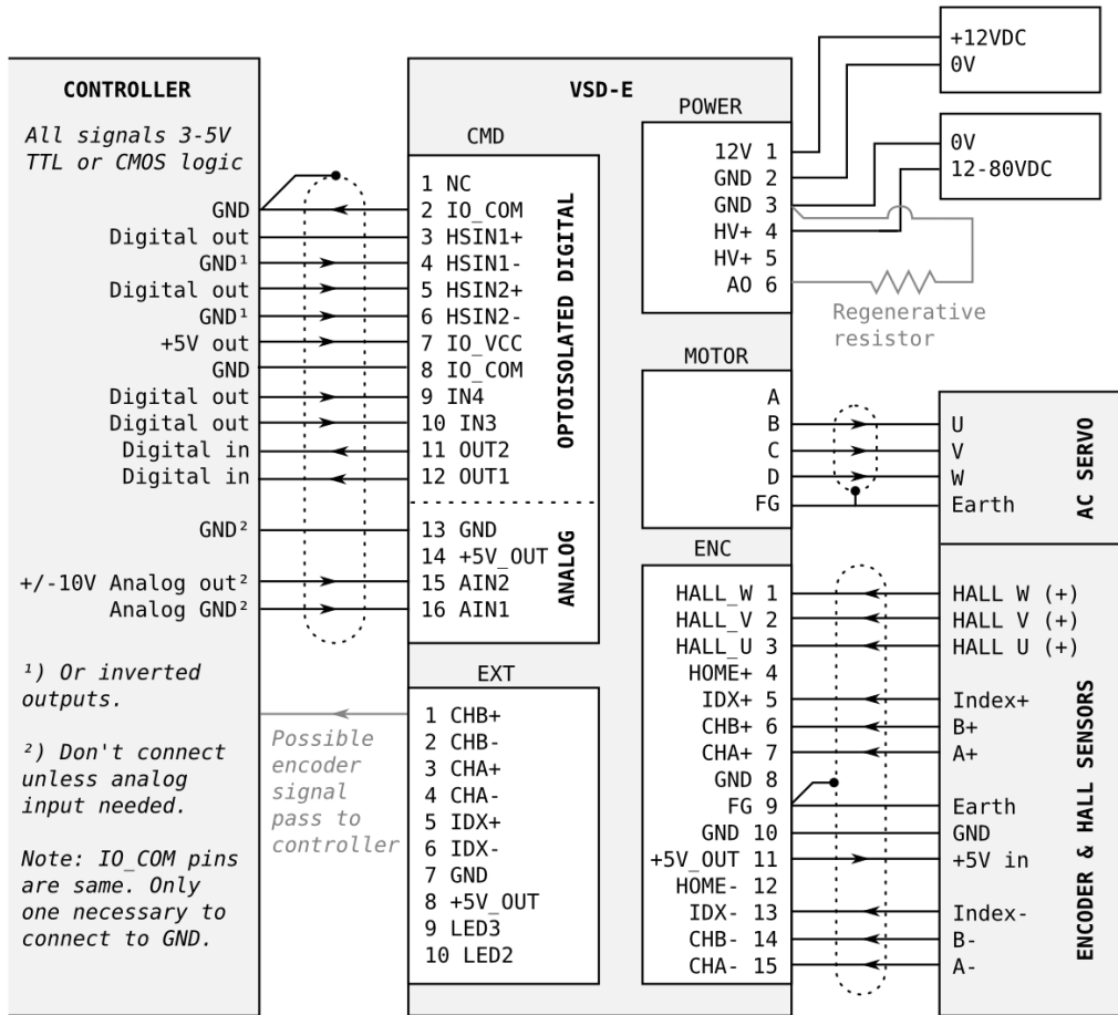
Figure 13: Typical controller and motor wiring. This configuration uses AC motor with Hall sensors. All of connections are not needed if certain features are not used.
